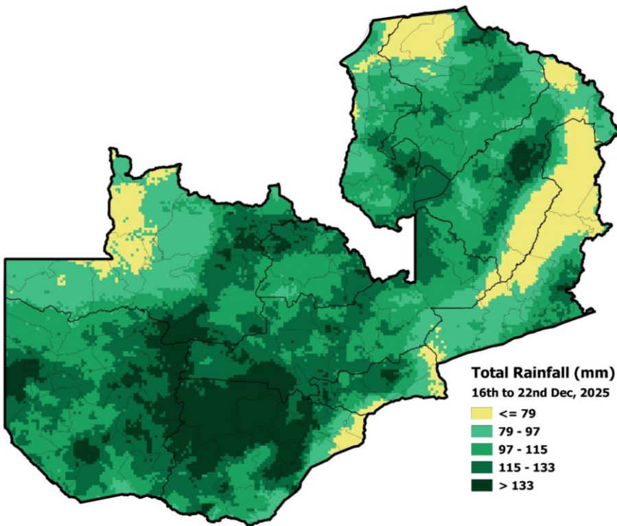
Figure 1: Forecasted total rainfall for the period 16 th to 22 nd Dec, 2025
