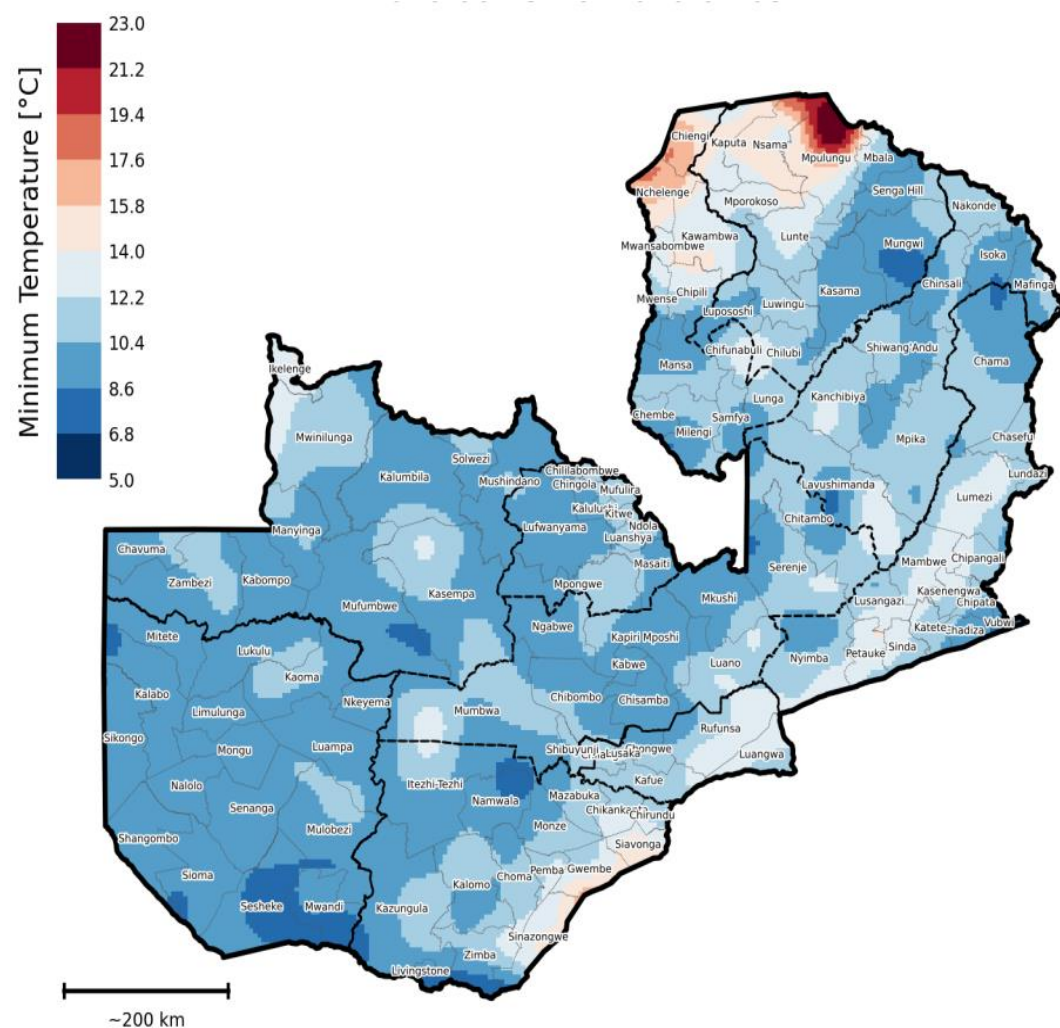
Figure 1: Minimum Temperature for the period 30th June to 6th July, 2026.
