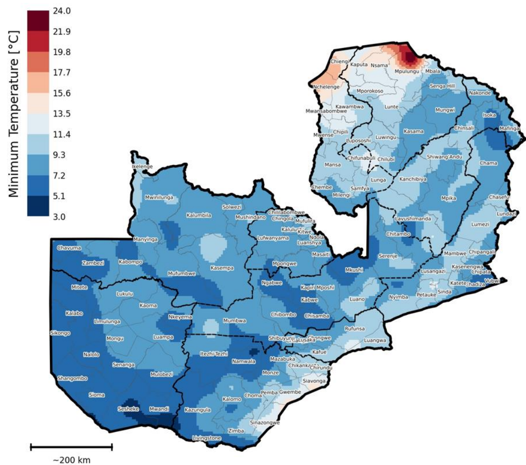
Figure 1: Minimum Temperature for the period 11th June to 17th July, 2026.
