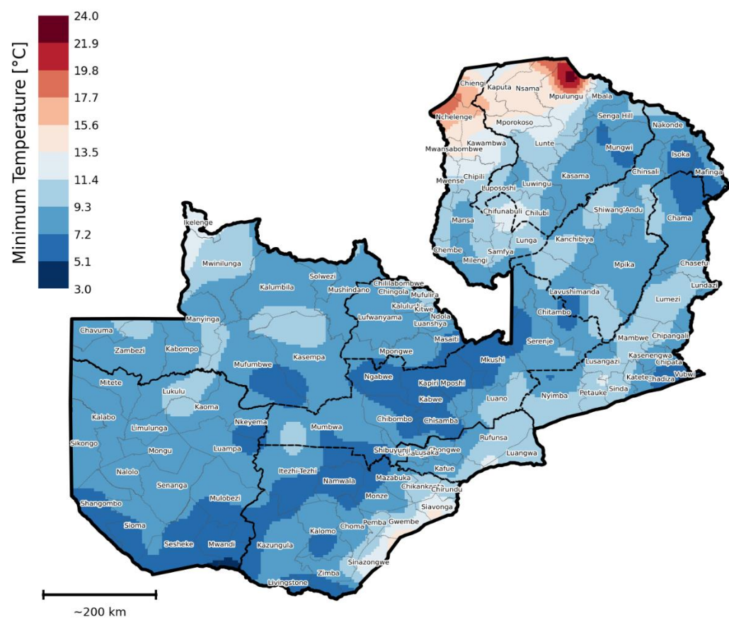
Figure 1: Minimum Temperature for the period 14th to 20th July, 2026.
