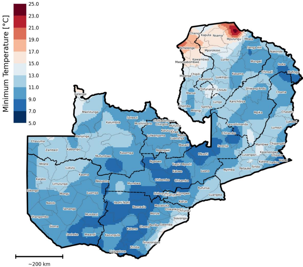
Figure 1: Minimum Temperature for the period 25th to 31st July, 2026.
