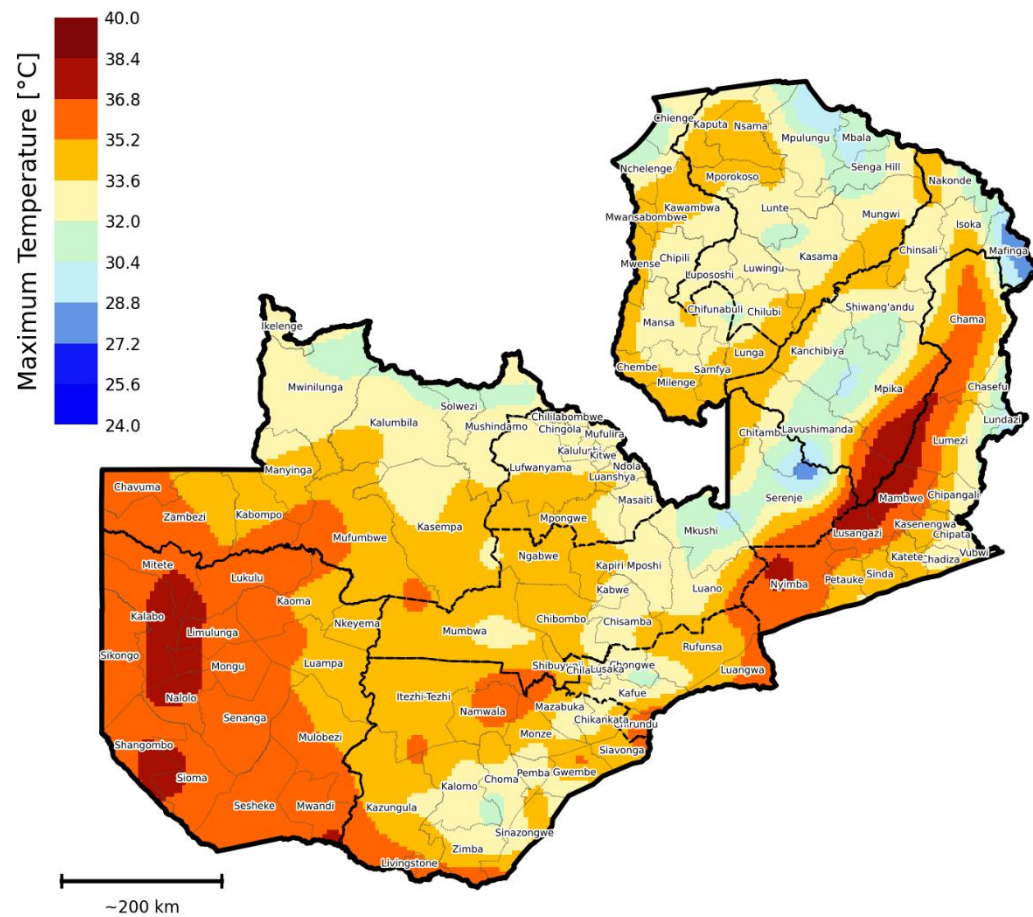
Figure 1: Maximum Temperature for the period 22 nd to 28 th September, 2026
