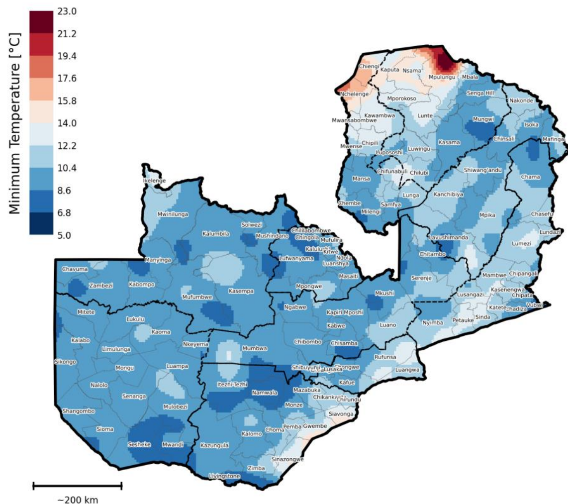
Figure 1: Minimum Temperature for the period 27th June to 3rd July, 2026
